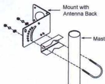
fig: Mounting Guide
